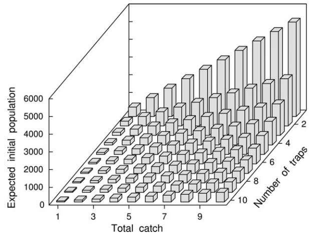
Fig. 3. Expected initial population of male pink bollworms flying at 1 \text{ m s}^{-1} for up to 10 h in a 100\text{-km}^2 area as related to the number of traps ( 2.61 \text{ m EAR}_c ) and the total catch on these traps (data generated from eqn 6).
